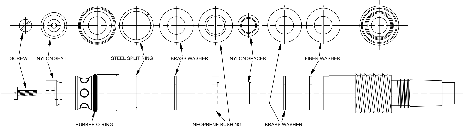
BODY - EXPLODED VIEW
